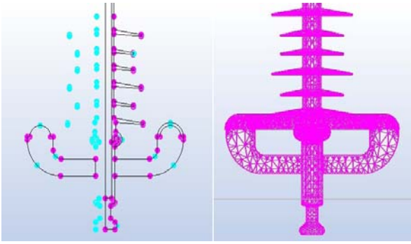
Fig. 3 2D view and 2D Triangular boundary elements assigned along Silicone Composite Insulator in COULOMB
