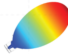
Far zone 3D pattern of electric field
