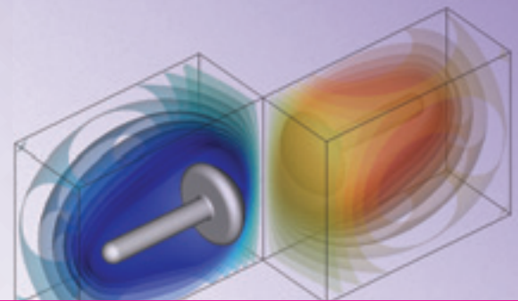
Voltage isosurfaces around mushroom electrodes
